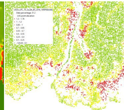
ground points
